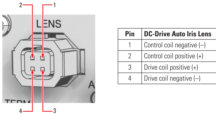
Figure 2. DC-Drive Auto Iris Lens Connector
